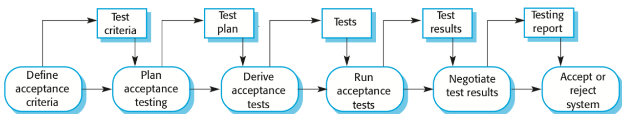
Figure 13-15: Acceptance Testing (Sommerville)
