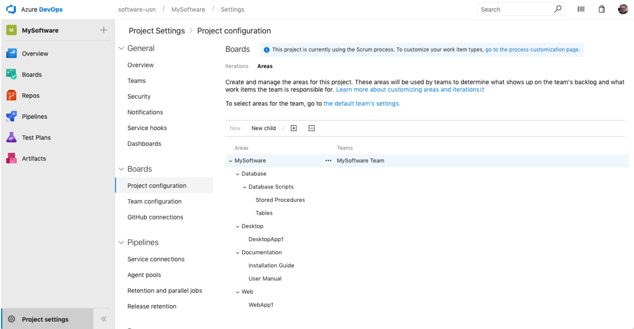
Figure 24-13: Configure Iterations and Sprints in Azure DevOps
